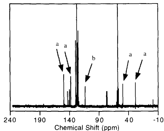
Figure 4. 13 C-NMR spectrum of blue solutions (UV/Vis spectrum showing an intense band at 605-nm) prepared by dissolving DPE (10 mg) in dimethyl sulfate (2 ml) containing H 2 SO 4 . The most characteristic carbons corresponding to the linear dimer 3 and DPE have been labelled with the letters a and b, respectively.
