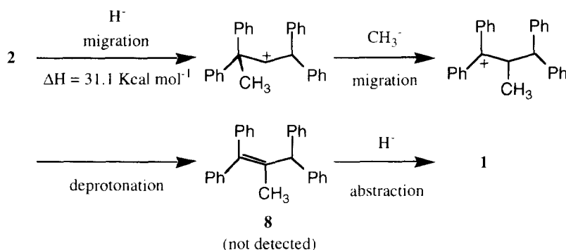
Scheme 2. Most reasonable pathway for allyl cation formation.
