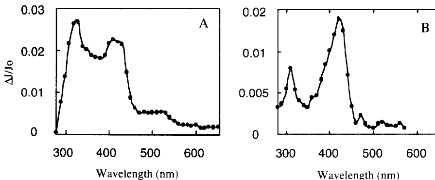
Figure 2. Transient spectrum of a solution of DPE in trifluoroethanol 1 \mu s after 266 nm excitation: A 30 min of N_2 purging; B purging with O_2 . The bands at 325, 430 and 520-nm can be assigned to DPEH^* , DPEH^+ and DPE^{+*} , respectively.
