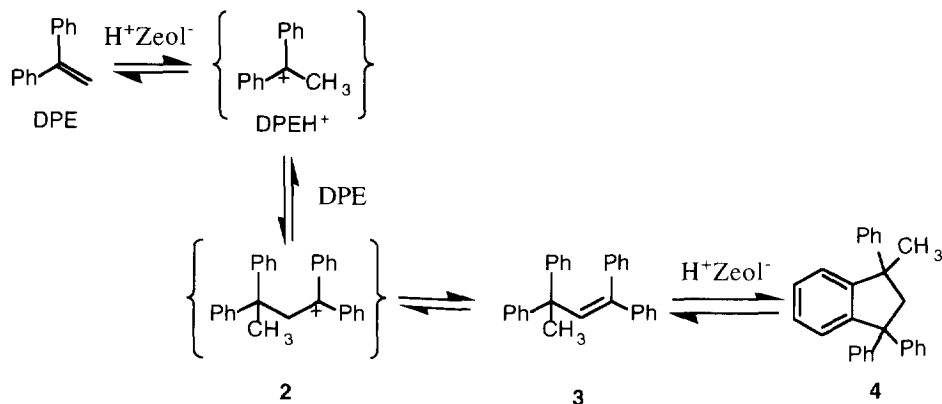
Scheme 1. Dimers observed after adsorption of DPE on acid zeolites.
