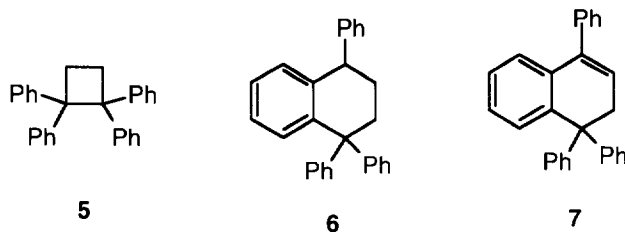
Chart 3. Characteristic dimers of an electron transfer mechanism.
