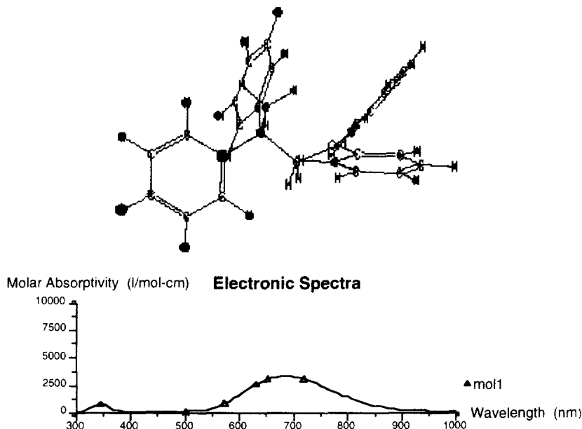
Figure 5. Optimized geometry of 1,1,3,3-tetraphenyl-1-butylium ion 2 . The size of the atomic radii has been plotted proportional to the local positive charge. The lower plot shows the ZINDO predicted UV/Vis spectrum for this cation where an absorption band in the visible is expected in contrast with the UV band ( \lambda < 500 -nm) calculated for DPEH + .
