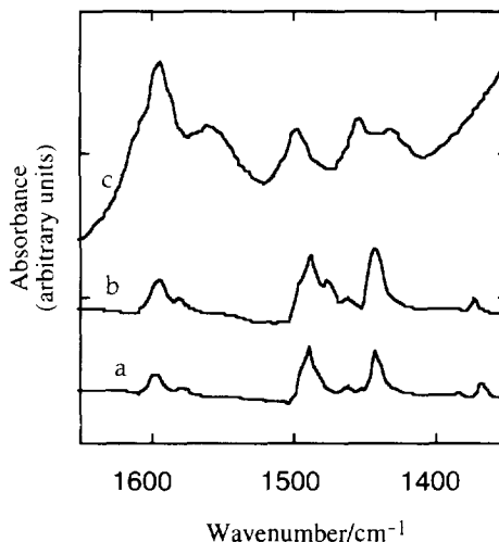
Figure 3. Aromatic region of the FT-IR Spectra of the linear dimer 3 (a) and the cyclic dimer 4 (b) in KBr disk. Spectrum c corresponds to the organic material present in the blue H \beta zeolite after incorporation of DPE. The last sample was outgassed at 100^\circ\text{C} under 10^{-2}\text{ Pa} for 1h prior to IR recording at room temperature.
